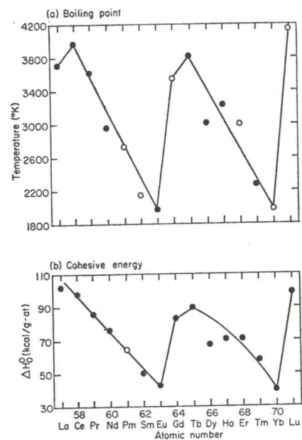
FIG. 16. (a) Boiling point of the rare-earth metals. (b) Cohesive energy of the rare-earth metals. Open points are estimated values.
